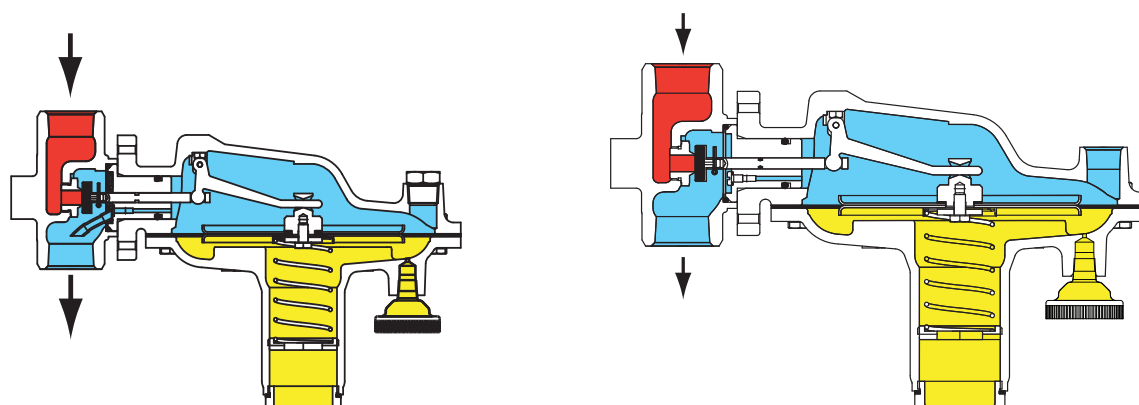
Fisher™ Type T205 with Internal Registration
