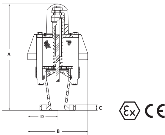
Figure 2. Enardo 961 Dimensions
