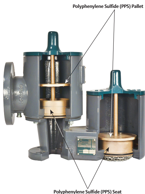
Figure 2. Enardo™ ES-850 Cut-Away View
