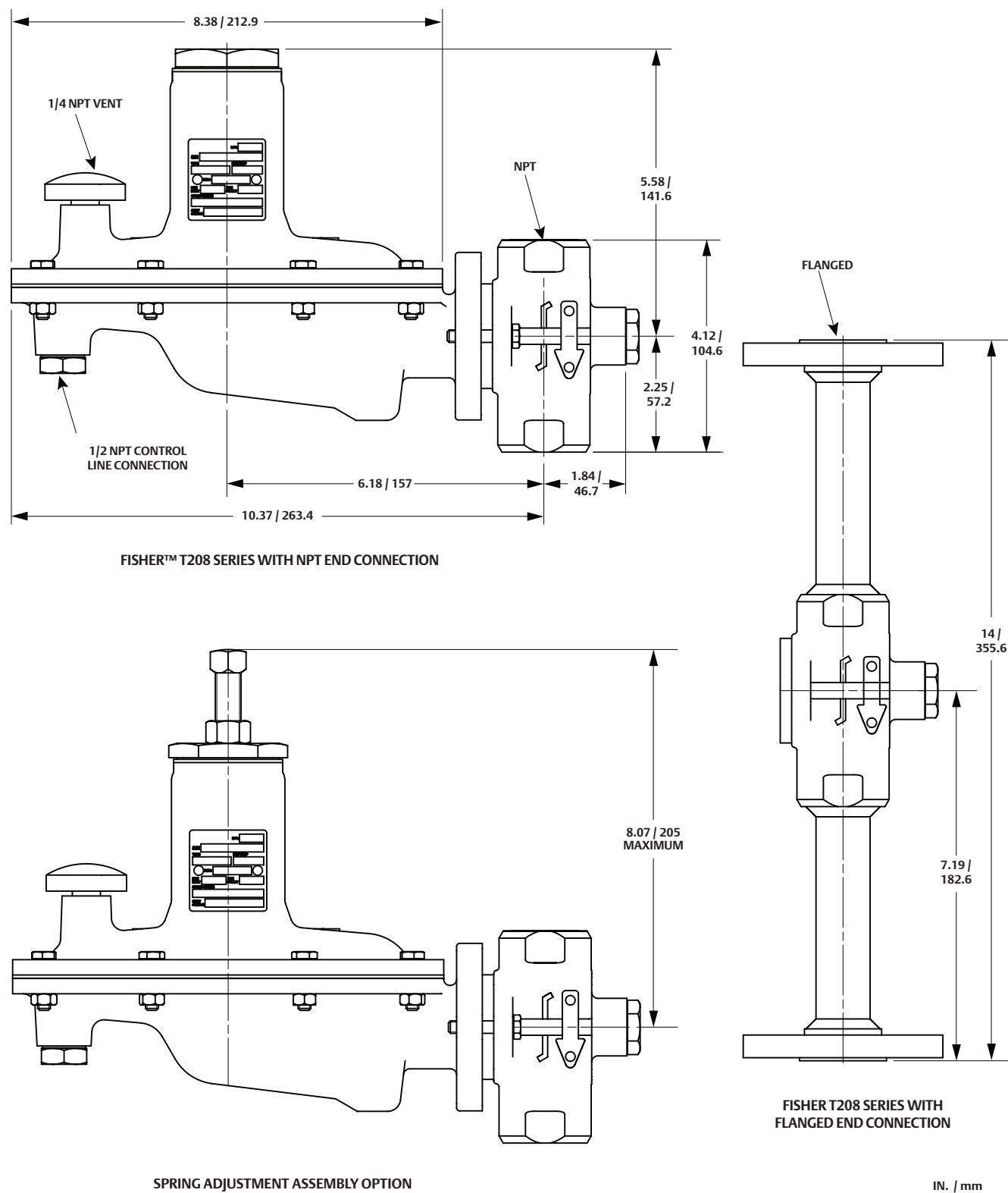
Figure 4. Dimensions
