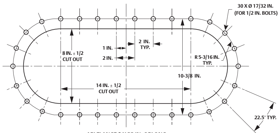
API FLANGE 8 X 22 IN. OBLONG
