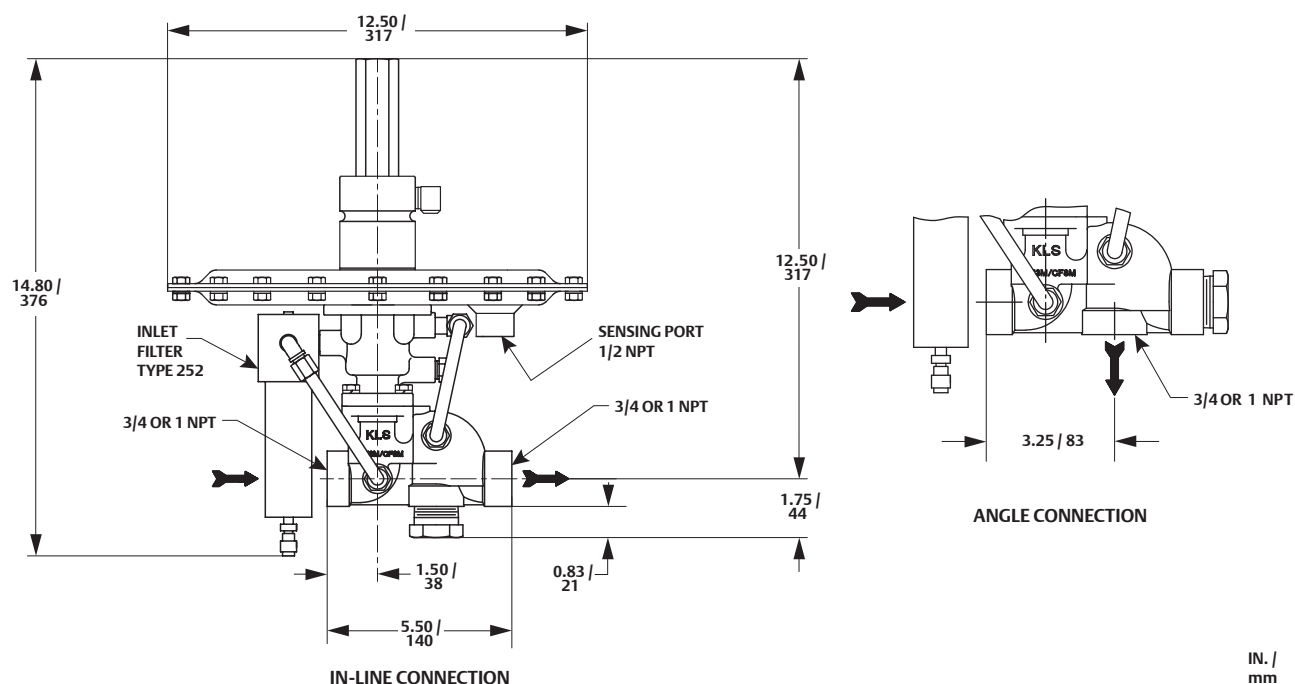
Figure 3. Dimensions
