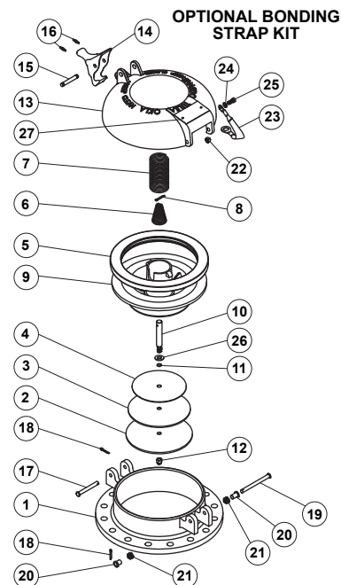
Figure 2. Enardo ES-665 Assembly Drawing
