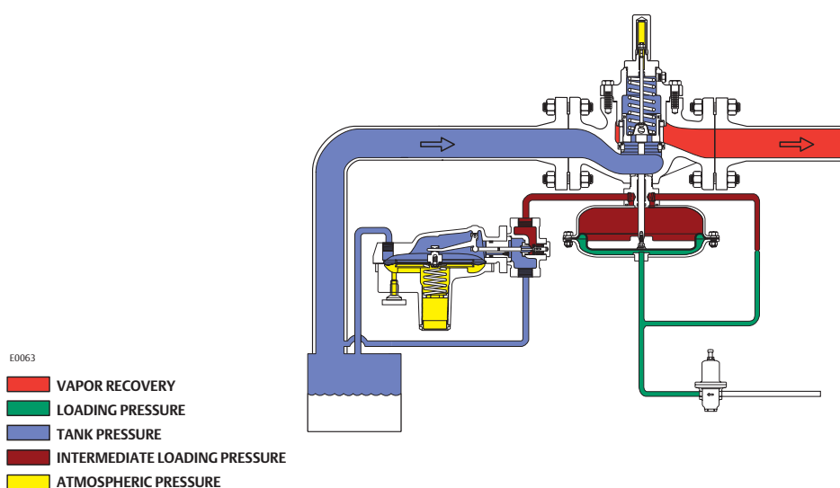
Figure 2. Operational Schematic
