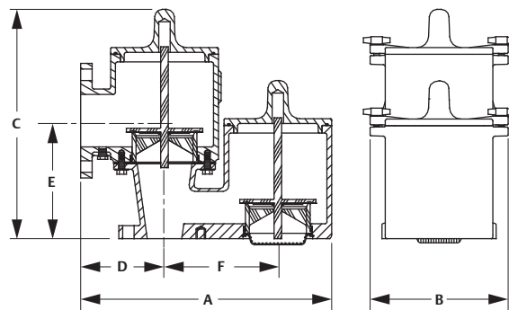
Figure 2. Enardo™ ES-850 Dimensions
