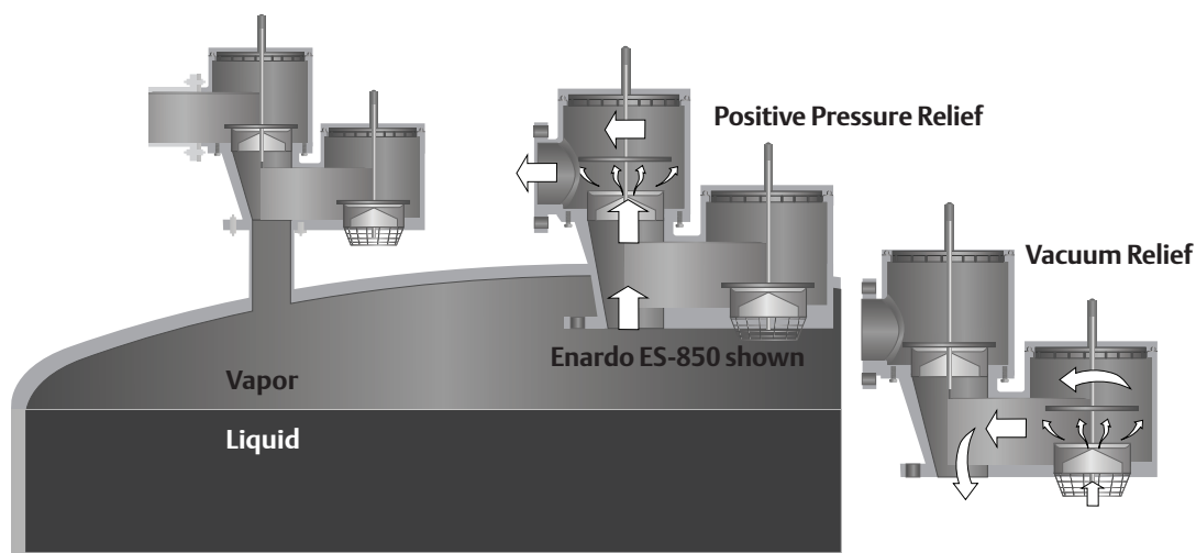
Figure 1. Enardo™ ES-850 Flow Illustration
