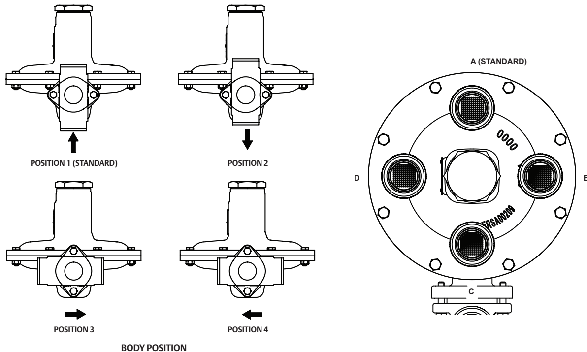
Figure 3. Body and Vent Orientation
