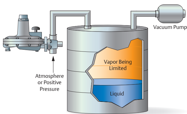
Figure 4. Vacuum Breakers
