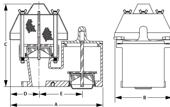
Figure 2. Enardo™ ES-950 Dimensions
