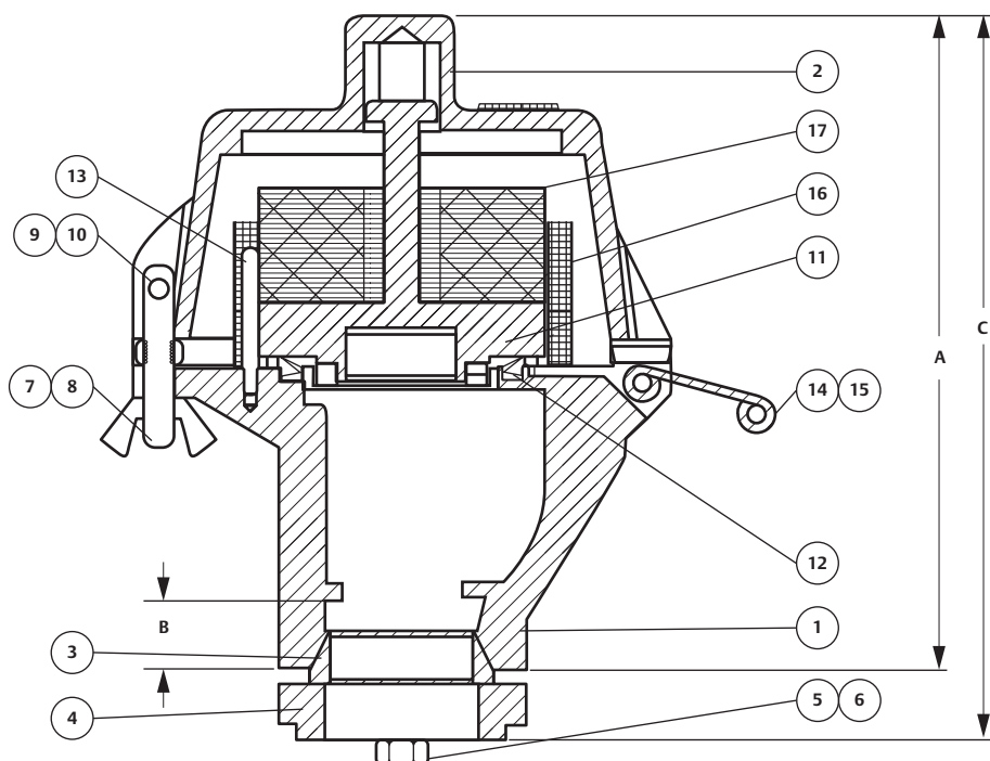
Figure 2. Enardo™ ES-905-SO Dimensions
