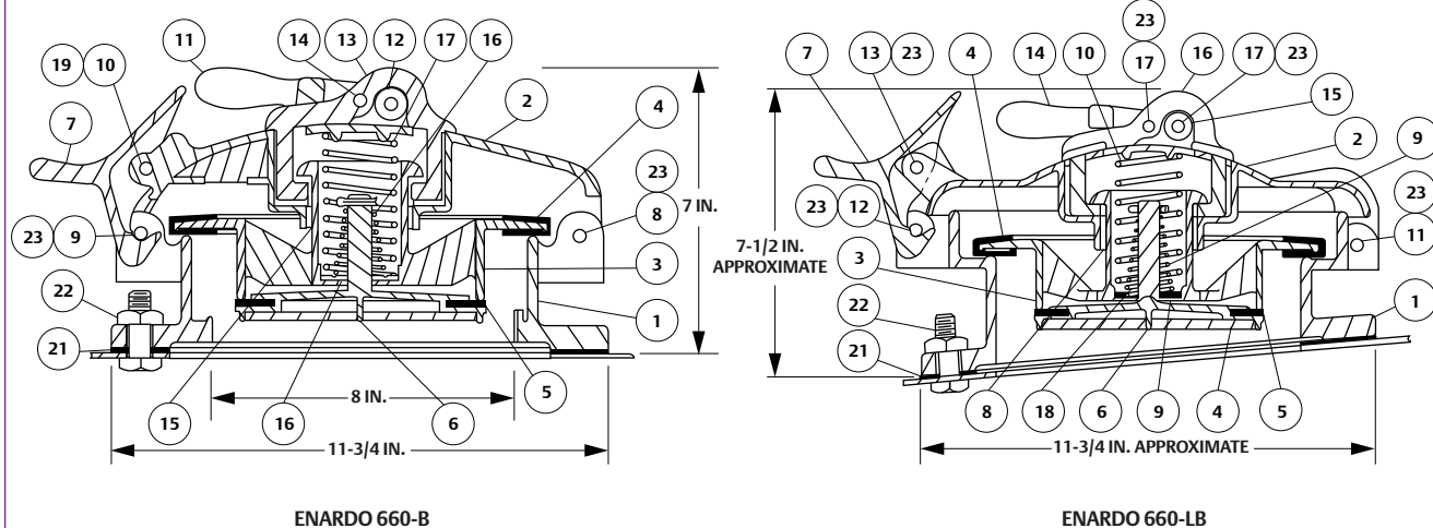
Figure 3. Enardo 660-B and Enardo 660-LB Assembly Drawings
